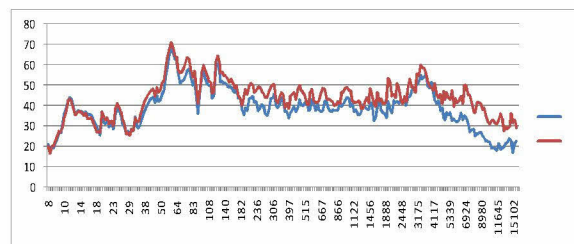
Freq. Response on a plasterboard panel DIN 120x100x8mm @1m (red line) e @2m (blue line)
